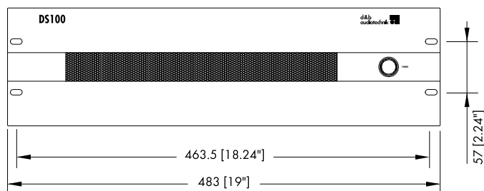
DS100 dimension in mm [inch]
